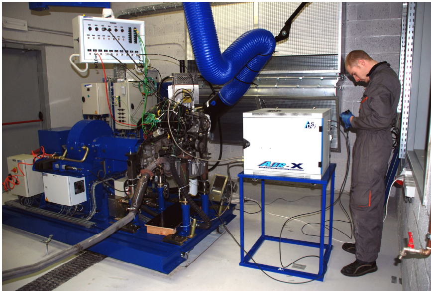
View on the sampling unit of Air-X installed in a test cell
